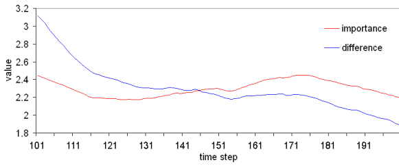
Fig. 11. The contrast between our importance measure and temporal difference with the earthquake data set, time steps 101 to 200.
